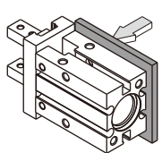
Front installation
