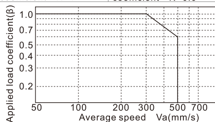
Fig 3: Applied load coefficient (β)
